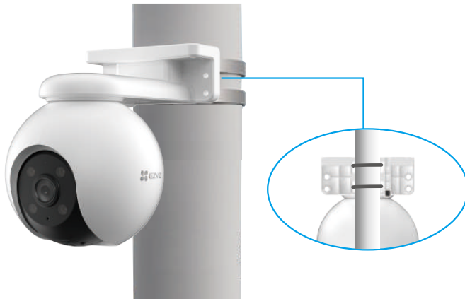
Fig.3 Pole Mount
