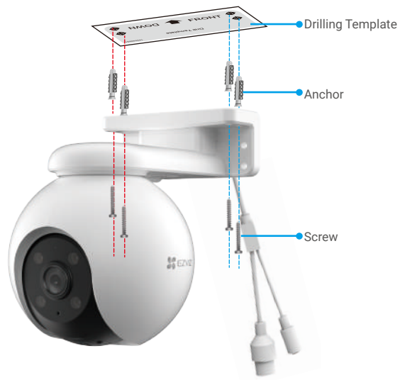
Fig. 1 Ceiling Mount
