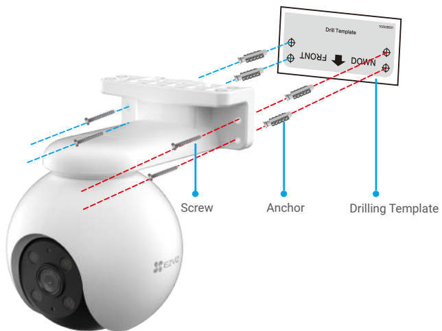
Fig. 2 Wall Mount
